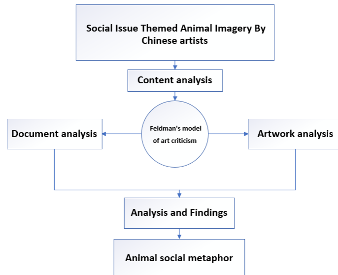
Fig. 1: Research framework
