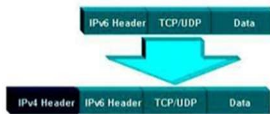
Figure 4. IPv6 over IPv4 Tunnelling (Meena & Bunde, 2015)
