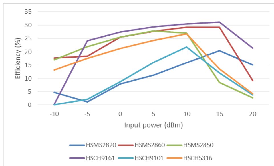
Figure 9. Efficiency of the proposed rectifier verses input RF power.
