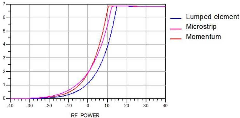
Figure 4. DC output voltage verses RF input power for voltage doubler rectifier circuit
