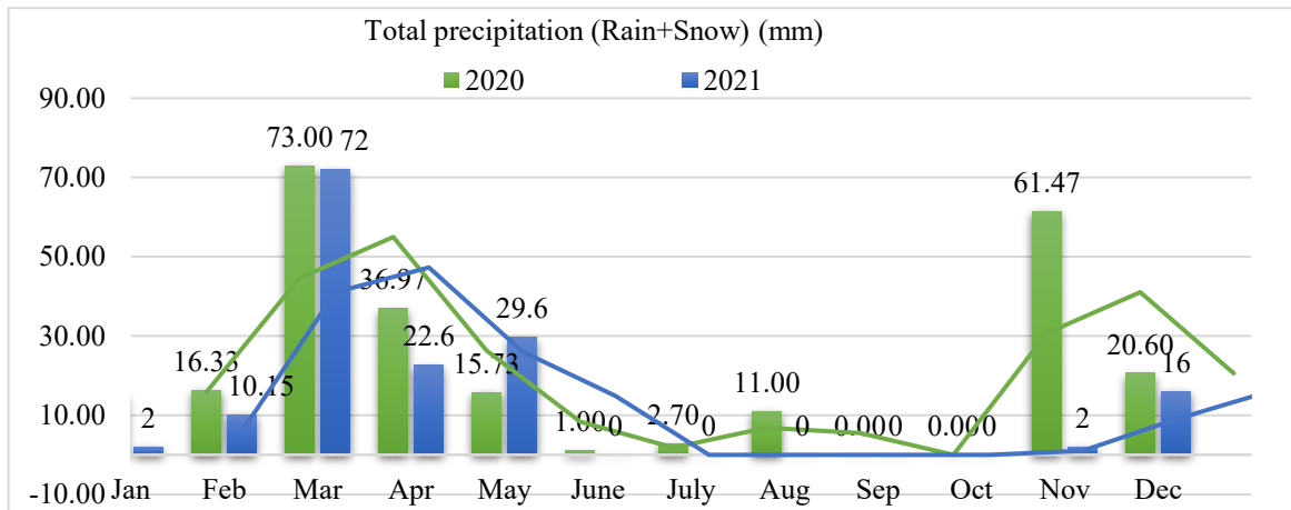
Fig. 2: Two annual meteorological data of precipitation (Rain Snow) (mm) in Kabul, Afghanistan, during the growing seasons of spring wheat in (2020 – 2021)
