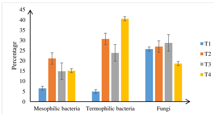
Fig. 2. Percentage of diversity microorganisms; mesophilic, thermophilic, and fungi in each pile of compost treatments.
